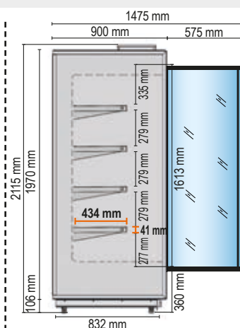
STROMBOLI 90 - SL Spalle cieche / Blind side walls SL Salumi e Latticini Cold cuts and Dairy products
