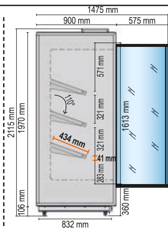
STROMBOLI 90 - FV Spalle cieche / Blind side walls FV Frutta e Verdura Fruit and Vegetables
