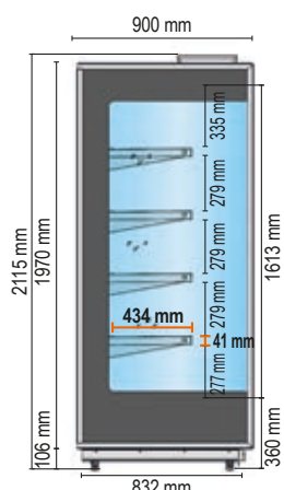
STROMBOLI 90 - C Spalle in vetrocamera temperato / Tempered double-glazed side walls C Carne preconfezionata Pre-packed meat
