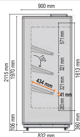
STROMBOLI 90 - FV Spalle cieche / Blind side walls FV Frutta e Verdura Fruit and Vegetables
