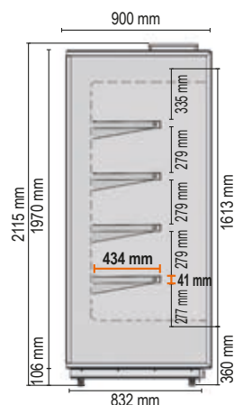
STROMBOLI 90 - SL Spalle cieche / Blind side walls SL Salumi e Latticini Cold cuts and Dairy products
