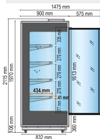
STROMBOLI 90 - SL Spalle in vetrocamera temperato / Tempered double-glazed side walls SL Salumi e Latticini Cold cuts and Dairy products
