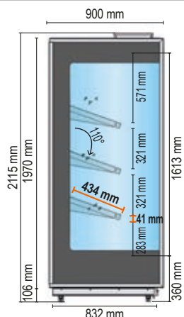
STROMBOLI 90 - FV Spalle in vetrocamera temperato / Tempered double-glazed side walls FV Frutta e Verdura Fruit and Vegetables
