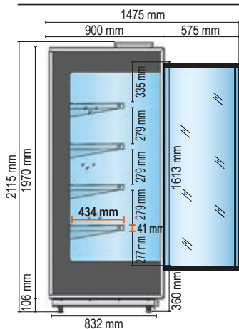
STROMBOLI 90 - C Spalle in vetrocamera temperato / Tempered double-glazed side walls C Carne preconfezionata Pre-packed meat
