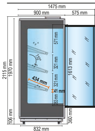
STROMBOLI 90 - FV Spalle in vetrocamera temperato / Tempered double-glazed side walls FV Frutta e Verdura Fruit and Vegetables
