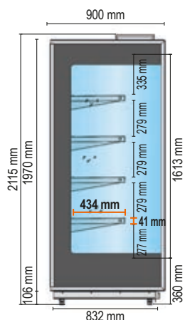
STROMBOLI 90 - SL Spalle in vetrocamera temperato / Tempered double-glazed side walls SL Salumi e Latticini Cold cuts and Dairy products
